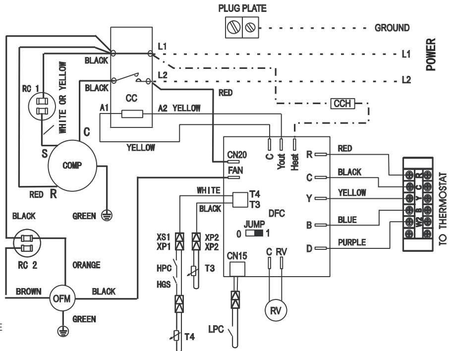
Fig.13 Outdoor Unit Wiring Diagram for H/P Systems(208/230V 1P 60Hz).
